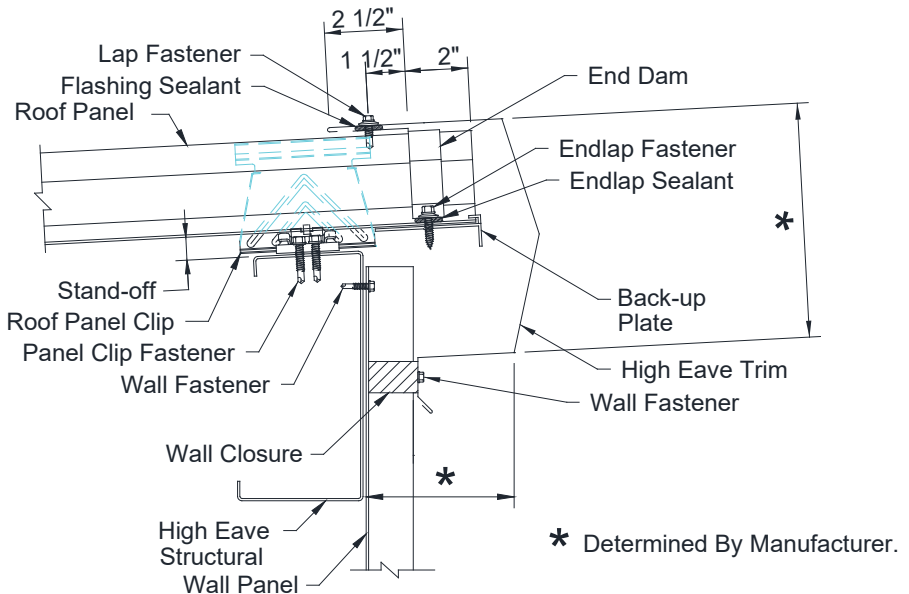
ALTERNATE HIGH EAVE SECTION - ORIGINAL BACK-UP PLATE
