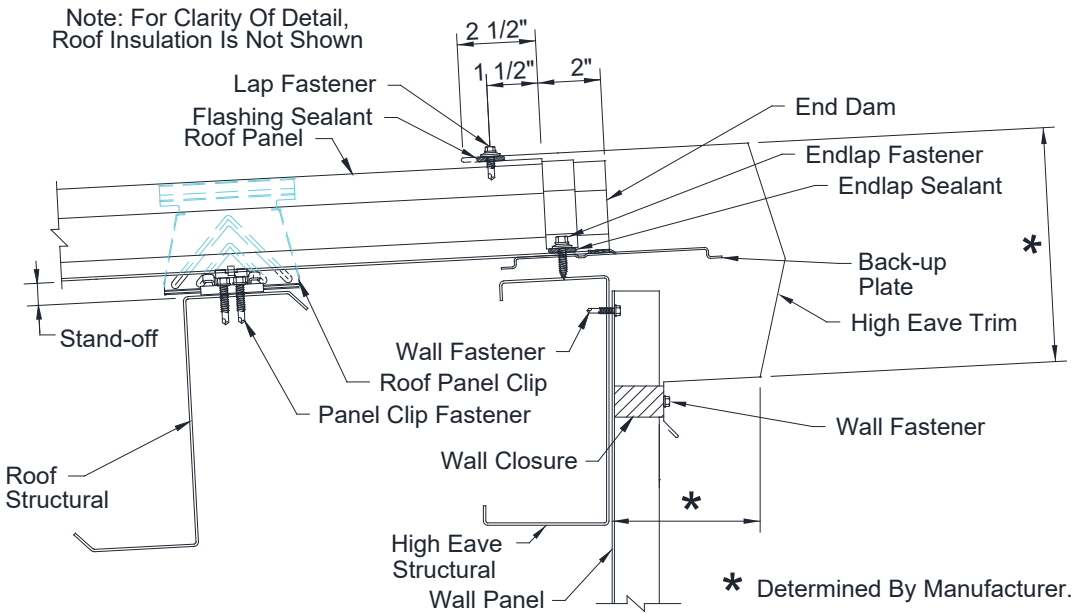
STANDARD HIGH EAVE SECTION - V.2 BACK-UP PLATE
