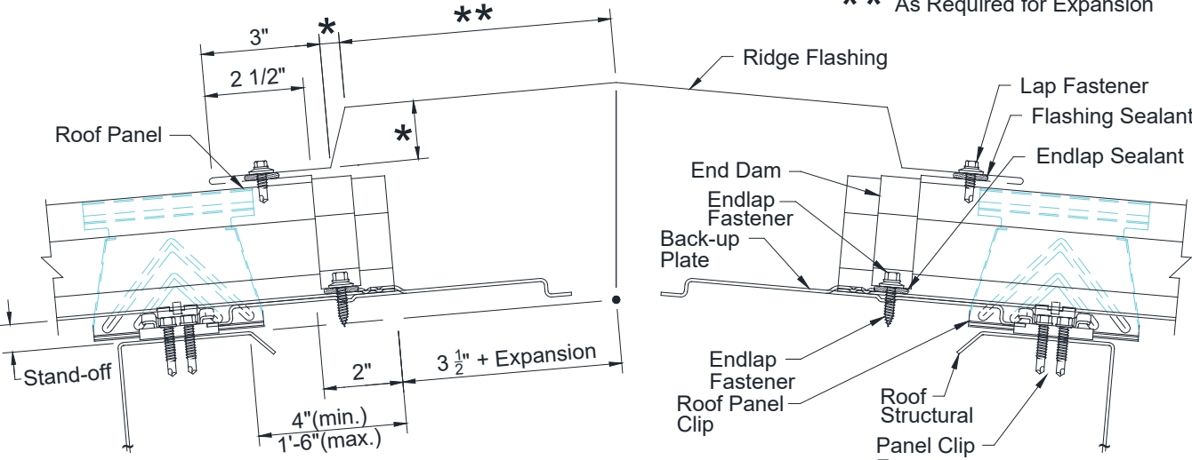
STANDARD RIDGE SECTION - V.2 BACK-UP PLATE
