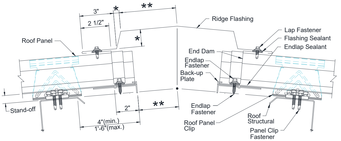
ALTERNATE RIDGE SECTION - ORIGINAL BACK-UP PLATE
