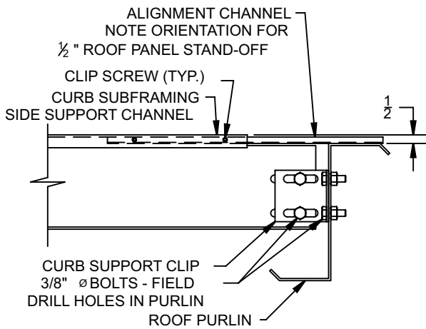
SECTION "A" 1/2" Roof panel Stand-off
