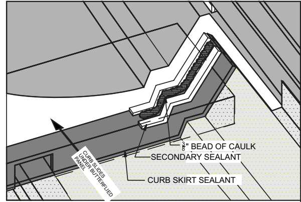
CORNER DETAIL
