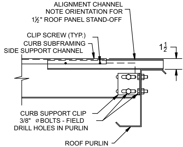
SECTION "A" 1 1/2" Roof panel Stand-off
